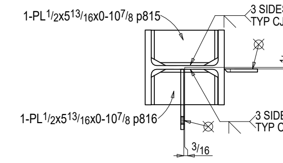
Section C-C 1C2
