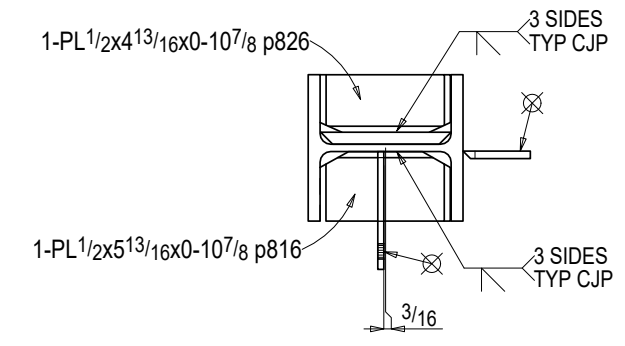
Section B-B 1C2
